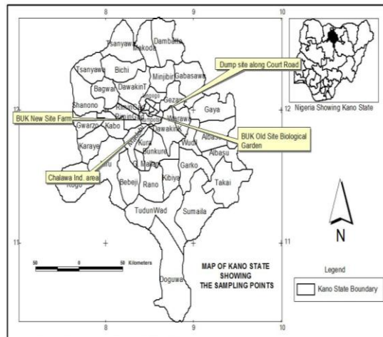
Fig. 4: Map of Kano State Showing the Sampling
