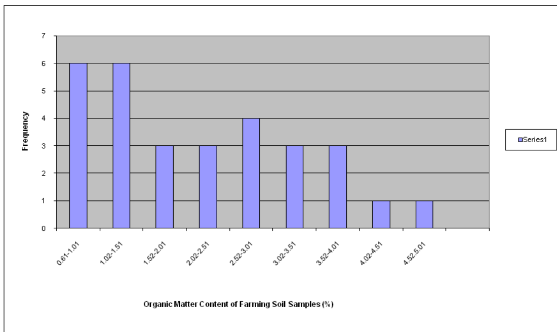
Fig. 9 : Frequency Distribution Pattern for Organic Matter Content of Farming Soil Samples
