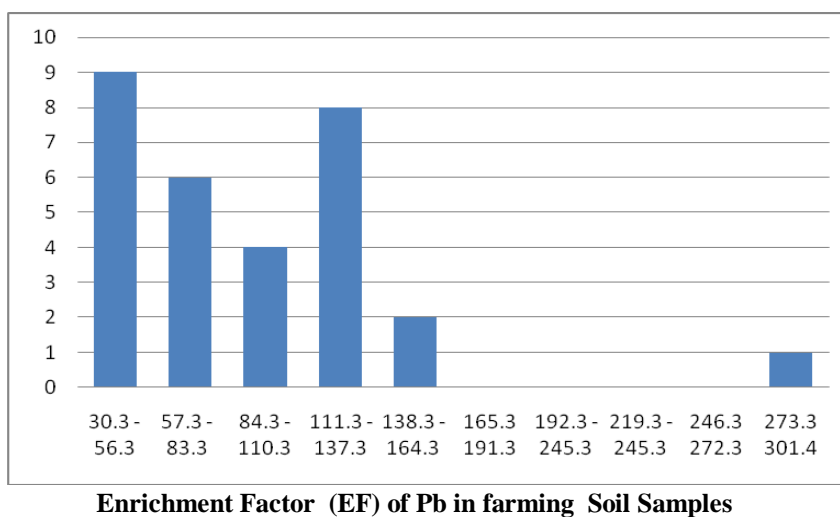
Figure 10: Frequency Distribution Pattern for Enrichment Factor of Pb in Farming Soil Samples, using Mn as a Reference Element
